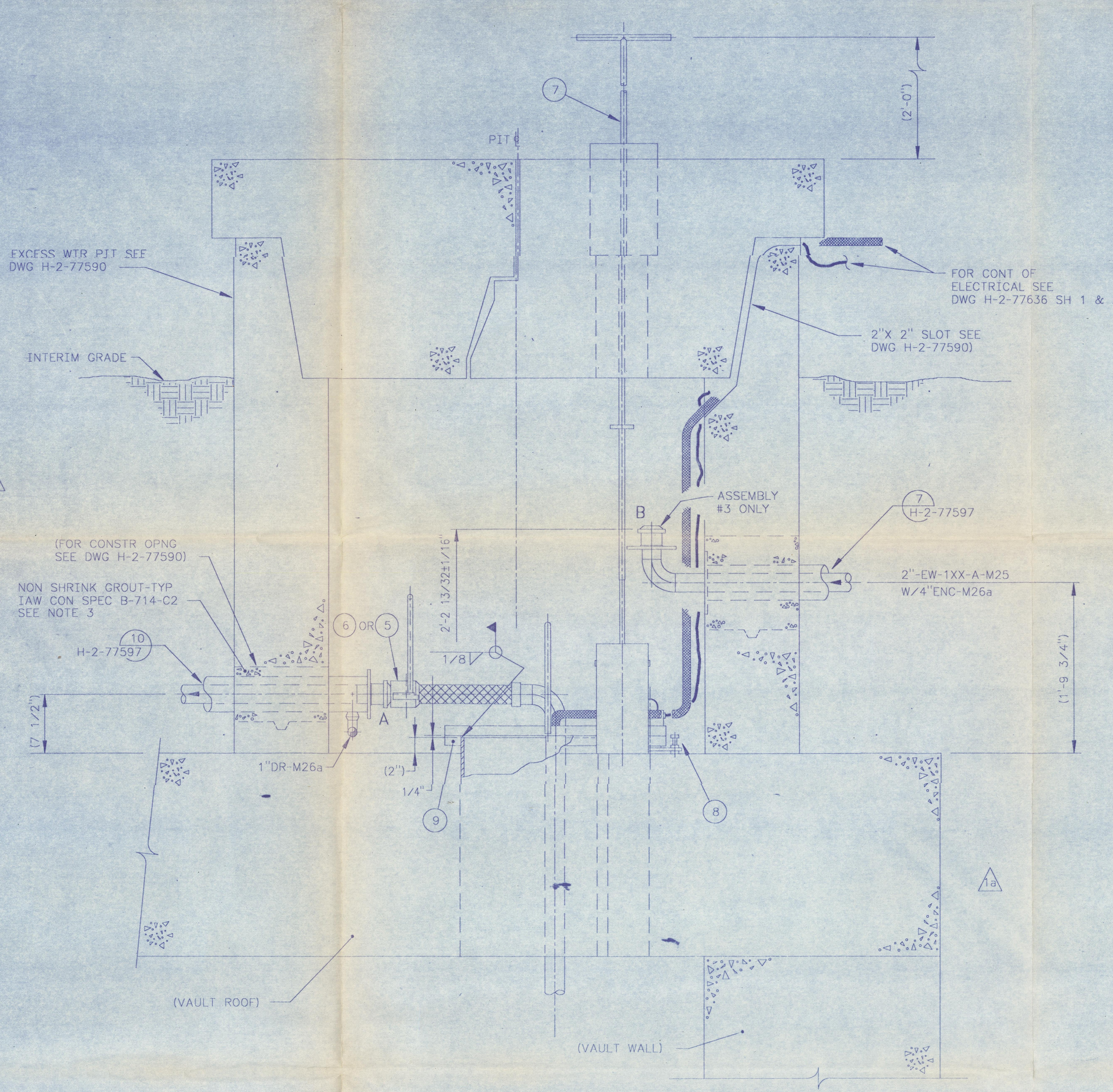
FOR EXCESS WTR PMP PIT PLAN, SECT, & DET SEE DWG H-2-77590 (ALTERNATE JUMPER ARRANGEMENT) PLAN (SIMILAR TO ASSY 3 ON SH 1)
