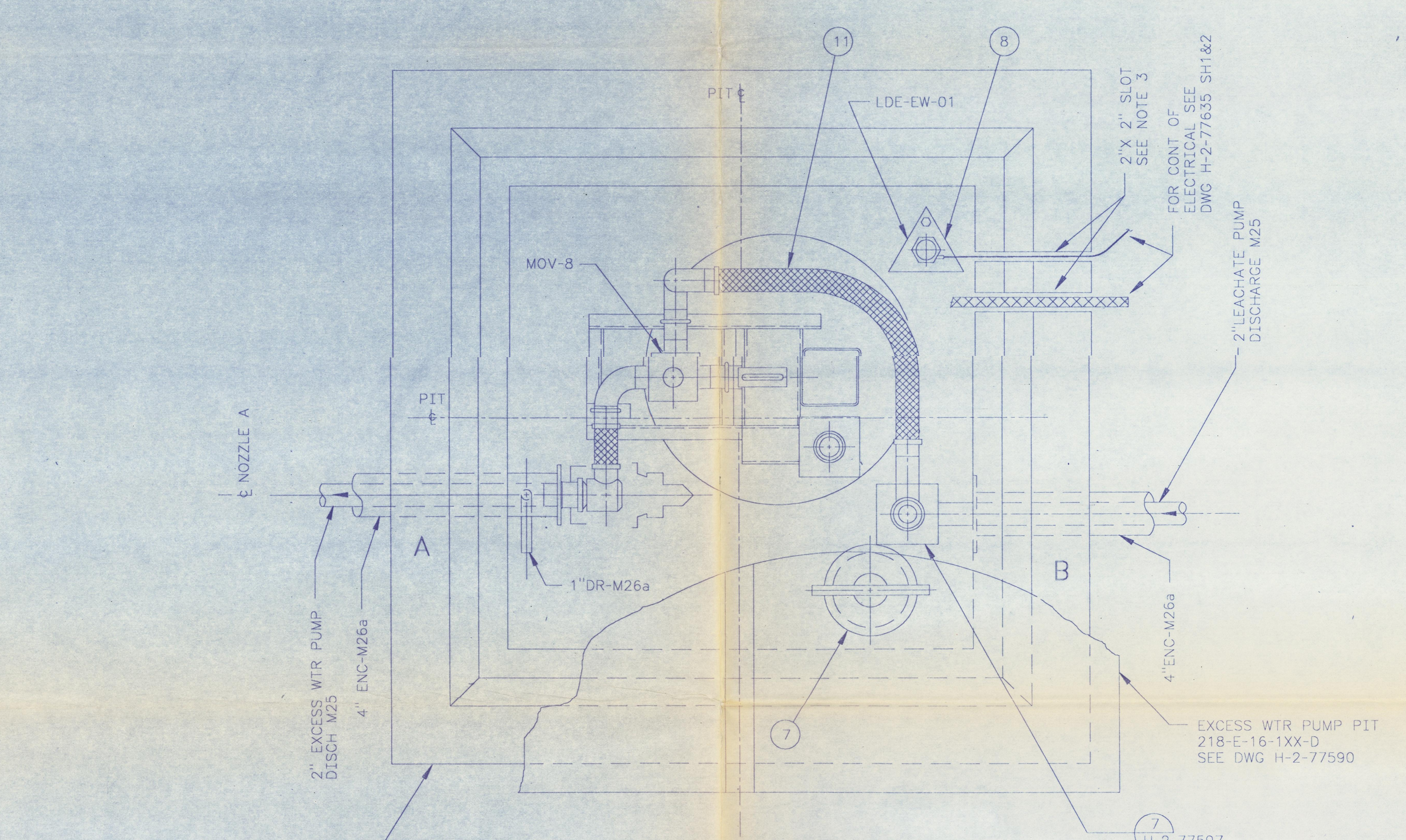
FOR EXCESS WTR PMP PIT PLAN, SECT, & DET SEE DWG H-2-77590 (ALTERNATE JUMPER ARRANGEMENT) PLAN (SIMILAR TO ASSY 3 ON SH 1)
