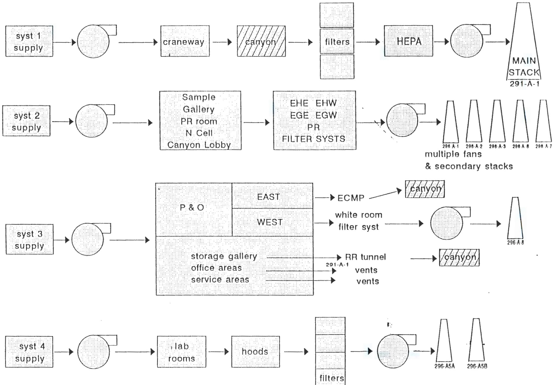
Figure 1: SIMPLIFIED EXISTING PUREX HVAC
