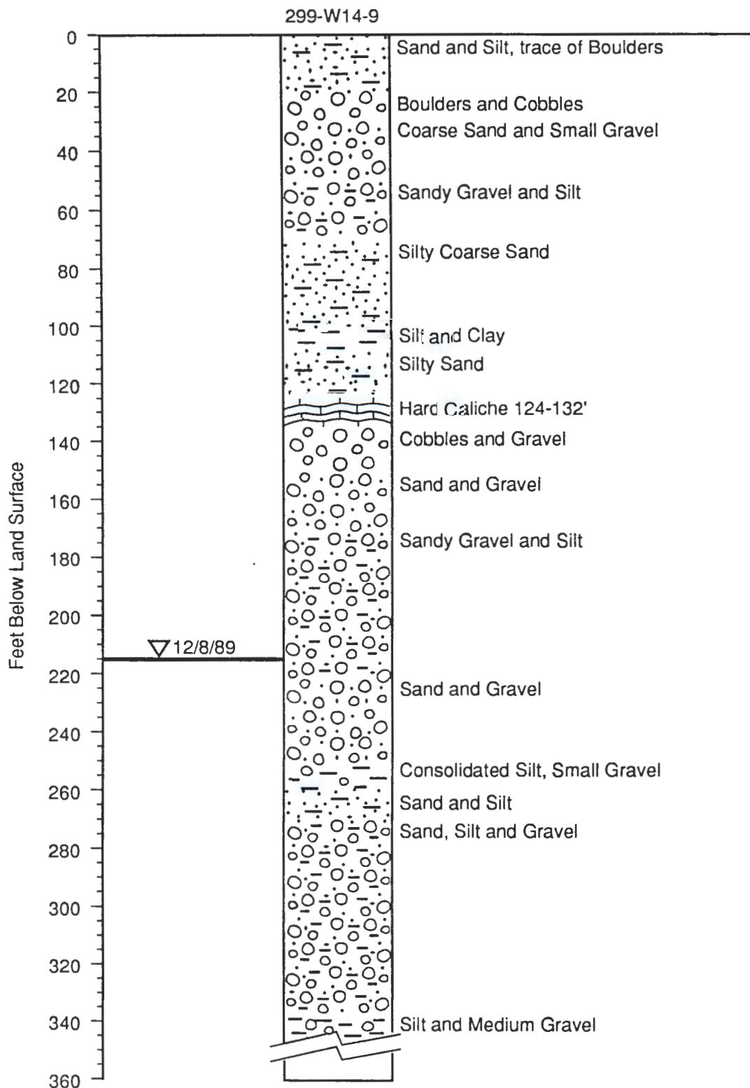
Figure 22. Lithology of Well 299-W14-9 South of the 284-WB Powerplant Ponds (WHC 1990a).
