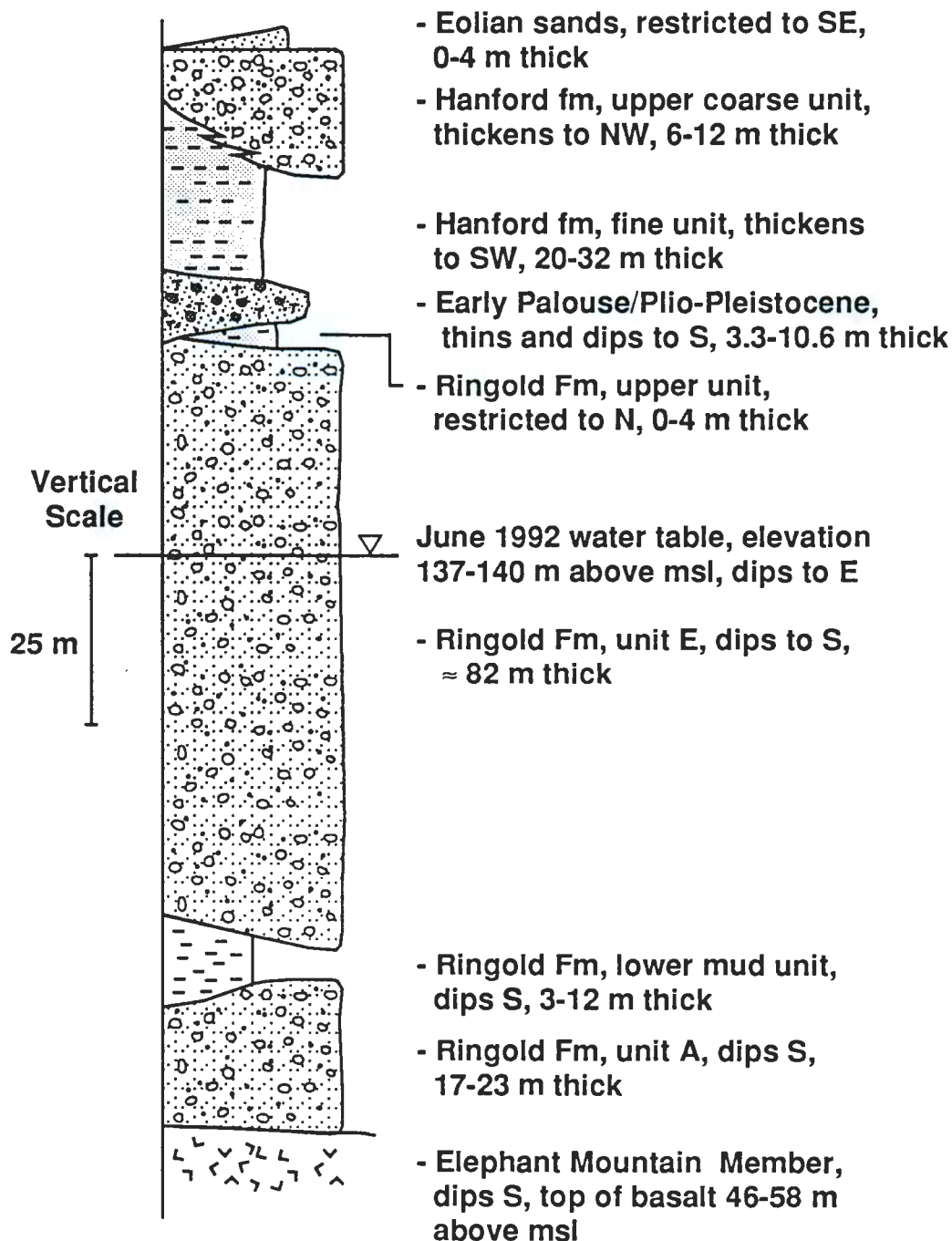
Figure 11. Generalized Stratigraphic Column for the Central 200 West Area.
