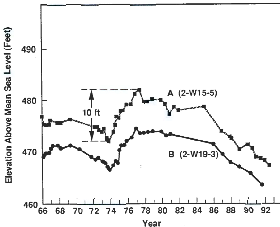
Figure 20. (a) Fluctuations in Water Table Elevations and (b) Correlation of Discharge History (In Wells South/Southwest of the 284-WB Powerplant Ponds).
