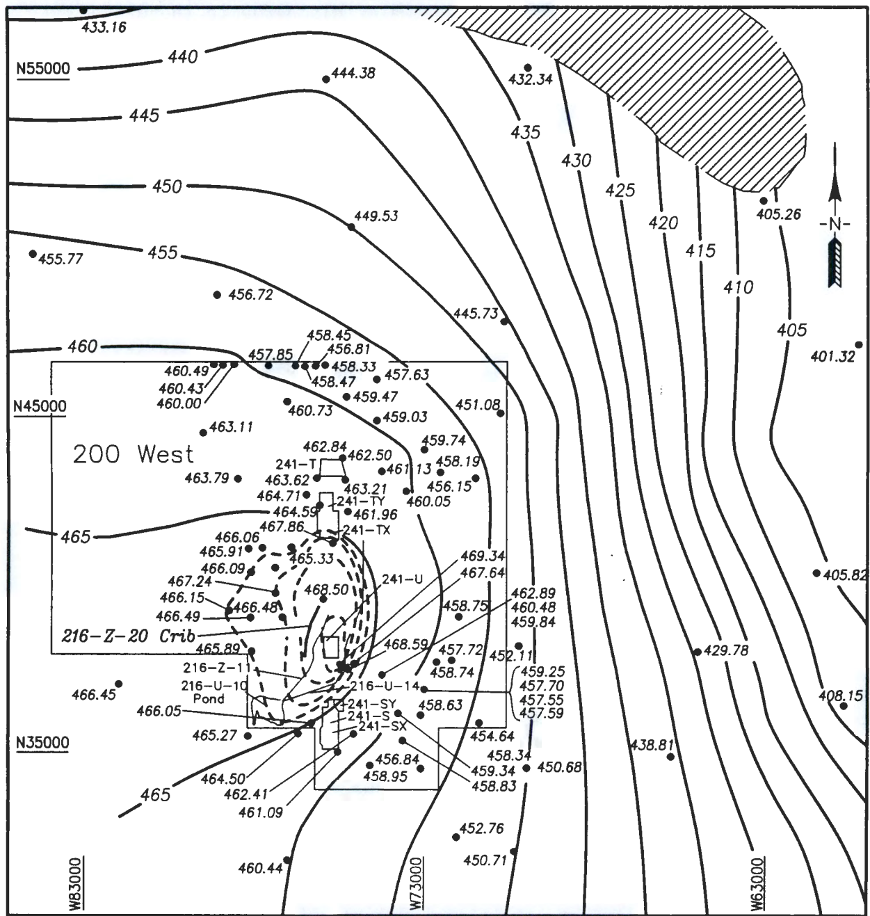
Figure 19. Water Table Map for 200 West Area and Surrounding Areas, December 1991.
