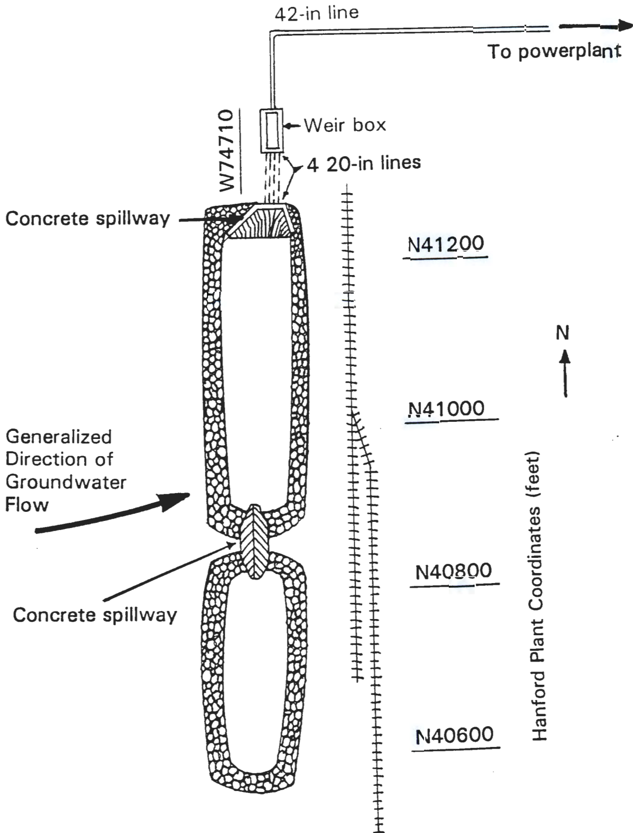
Figure 3. Plan View of the 284-WB Powerplant Ponds.
