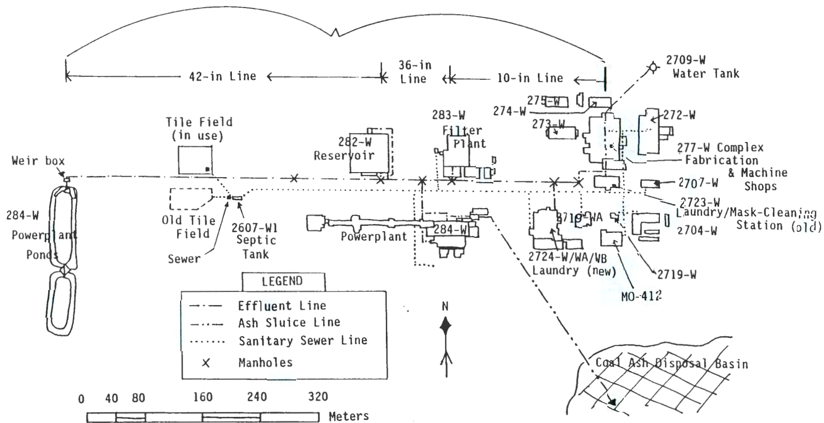
Figure 4. Schematic of 284-W Powerplant Effluent Line.
