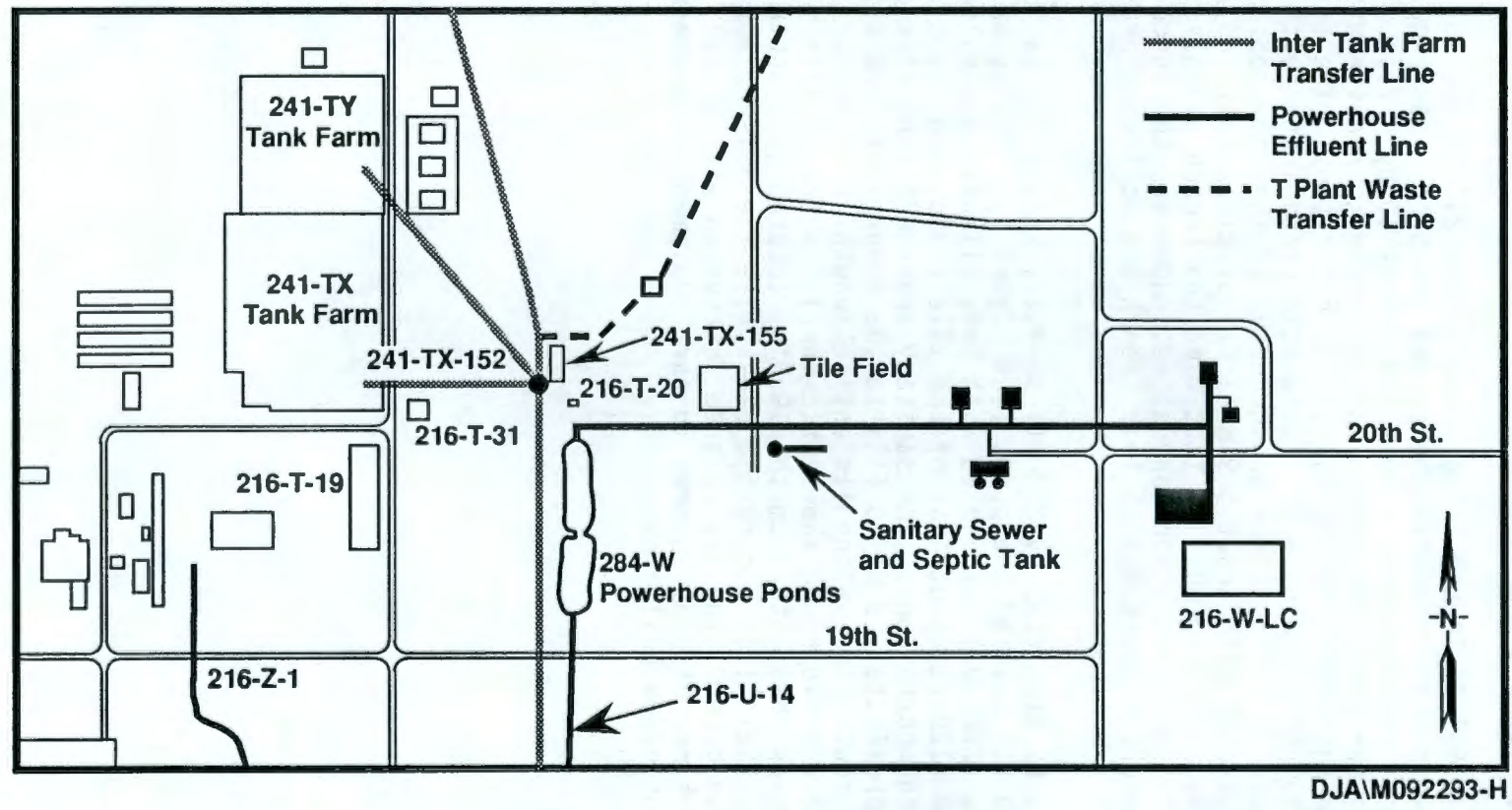
Figure 5. Location of Effluent Lines and Other Structures in the Vicinity of the 284-WB Powerplant Ponds.
