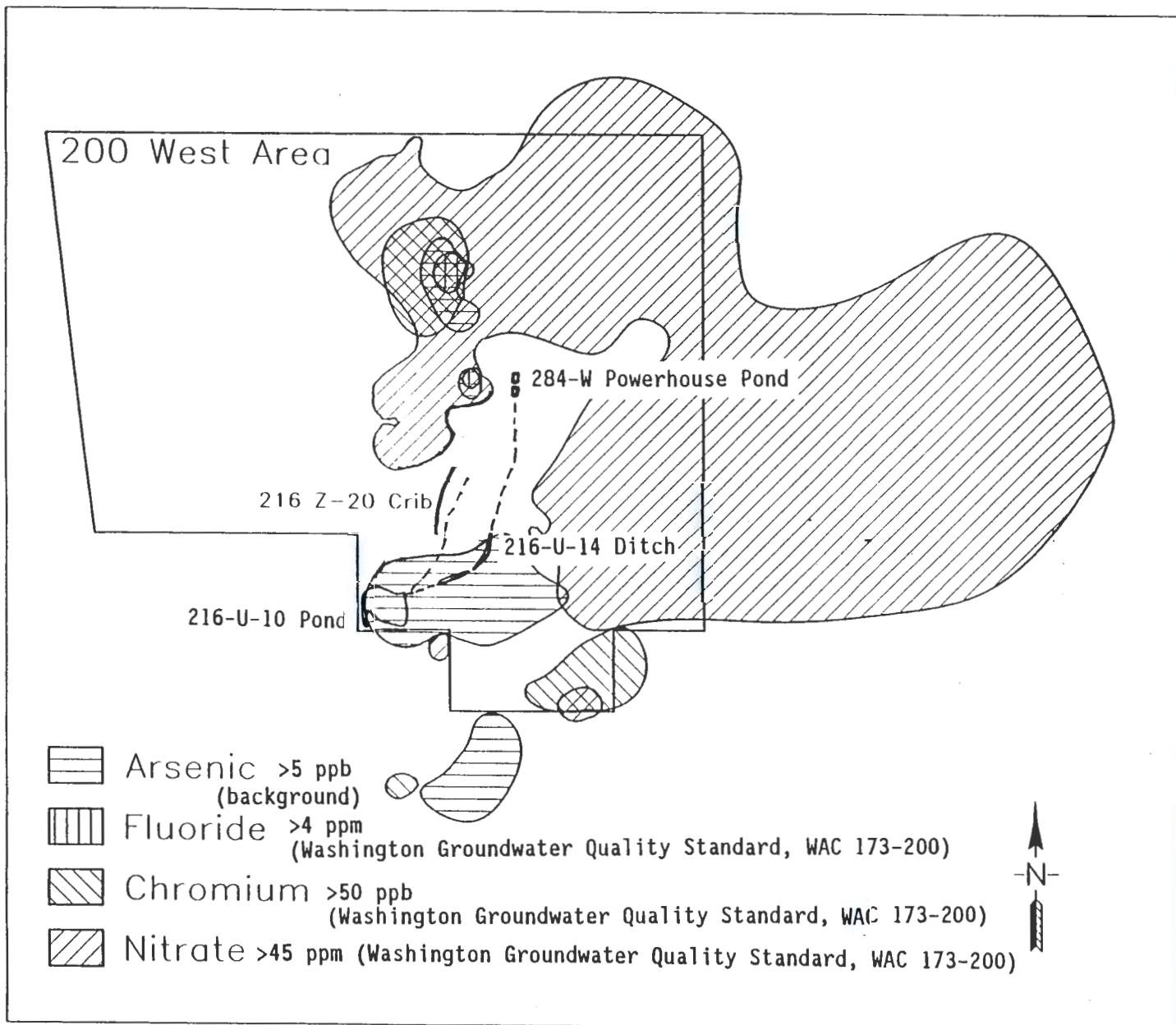
Figure 16. Contaminant Plume Map for Arsenic, Fluoride, Chromium, and Nitrate--200 West Area.
