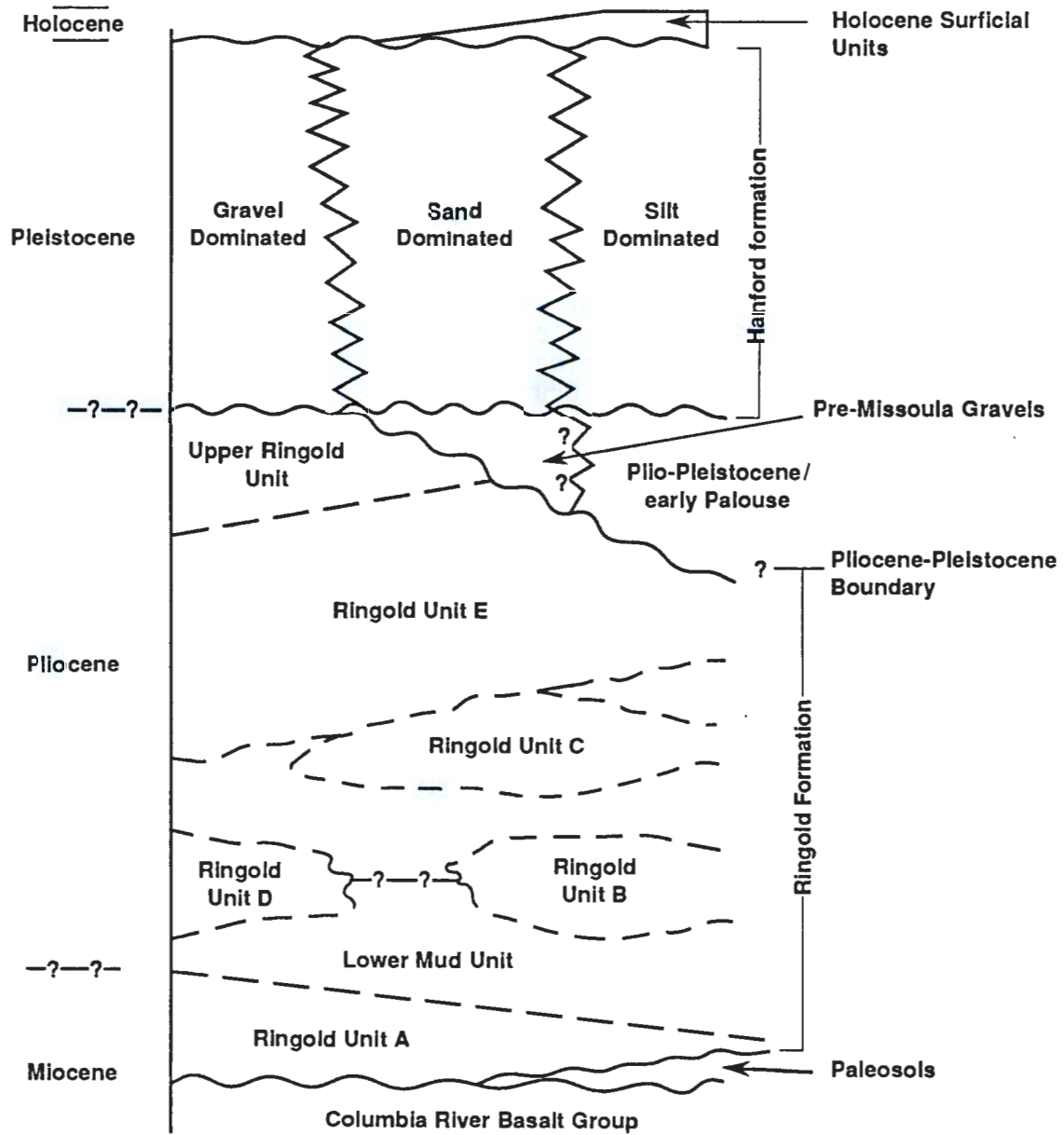
Figure 10. Generalized Stratigraphy of the Suprabasalt Sediments in the Pasco Basin.
