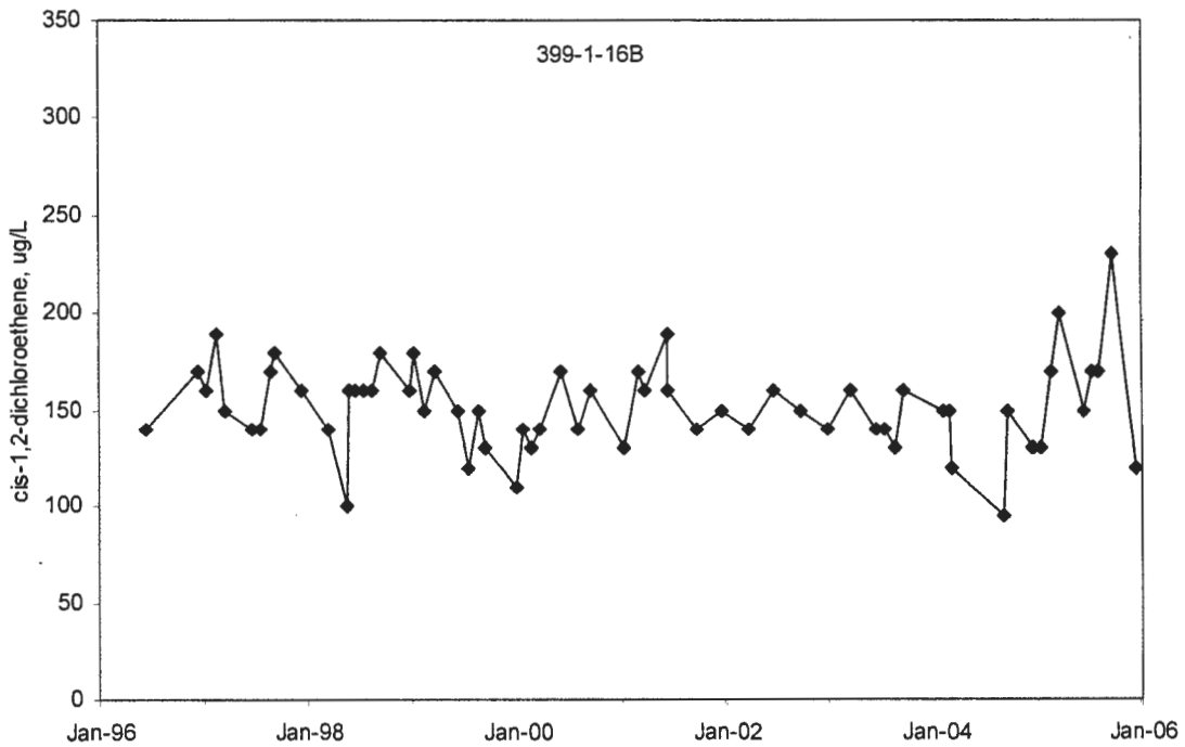
Figure 7. Cis-1,2-Dichloroethene Concentrations in Well 399-1-16B
