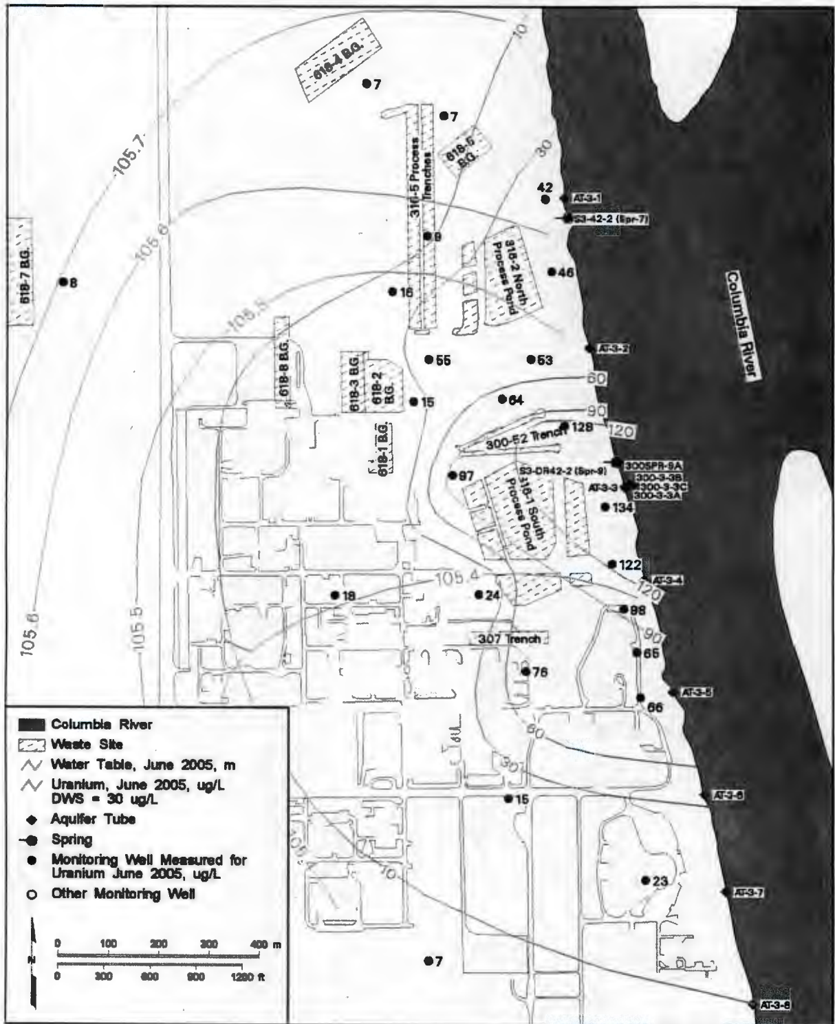
Figure 2. Uranium Concentrations in the Upper Portion of the Unconfined Aquifer, June 2005 (Hartman et al. 2006).
