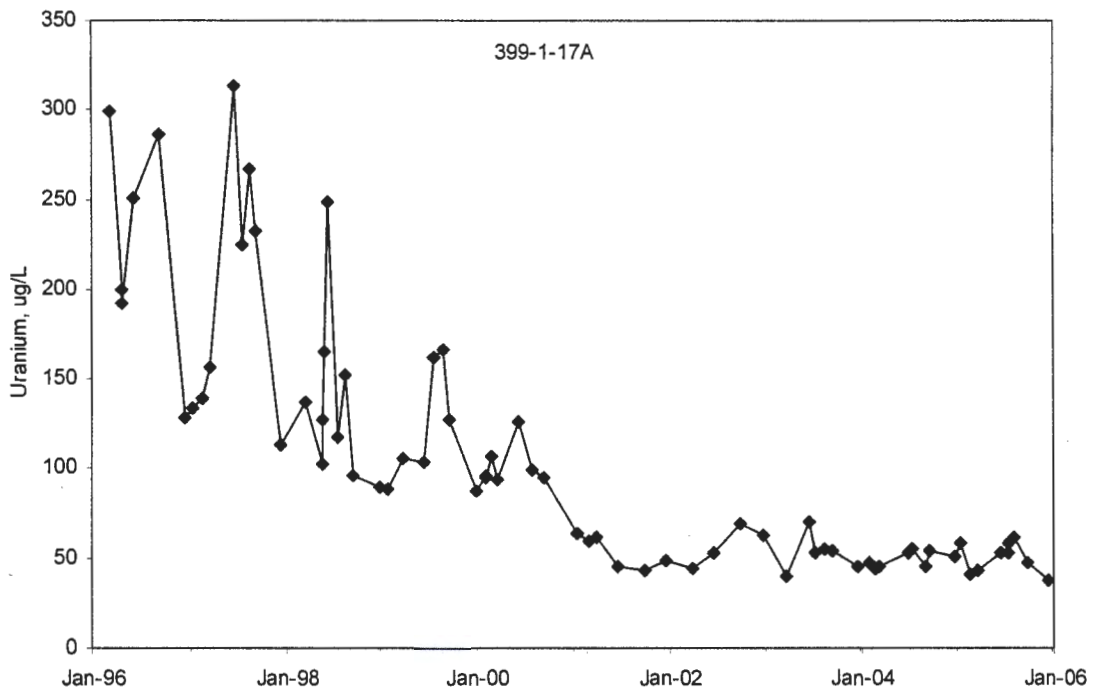
Figure 6. Uranium Concentrations in Well 399-1-17A
