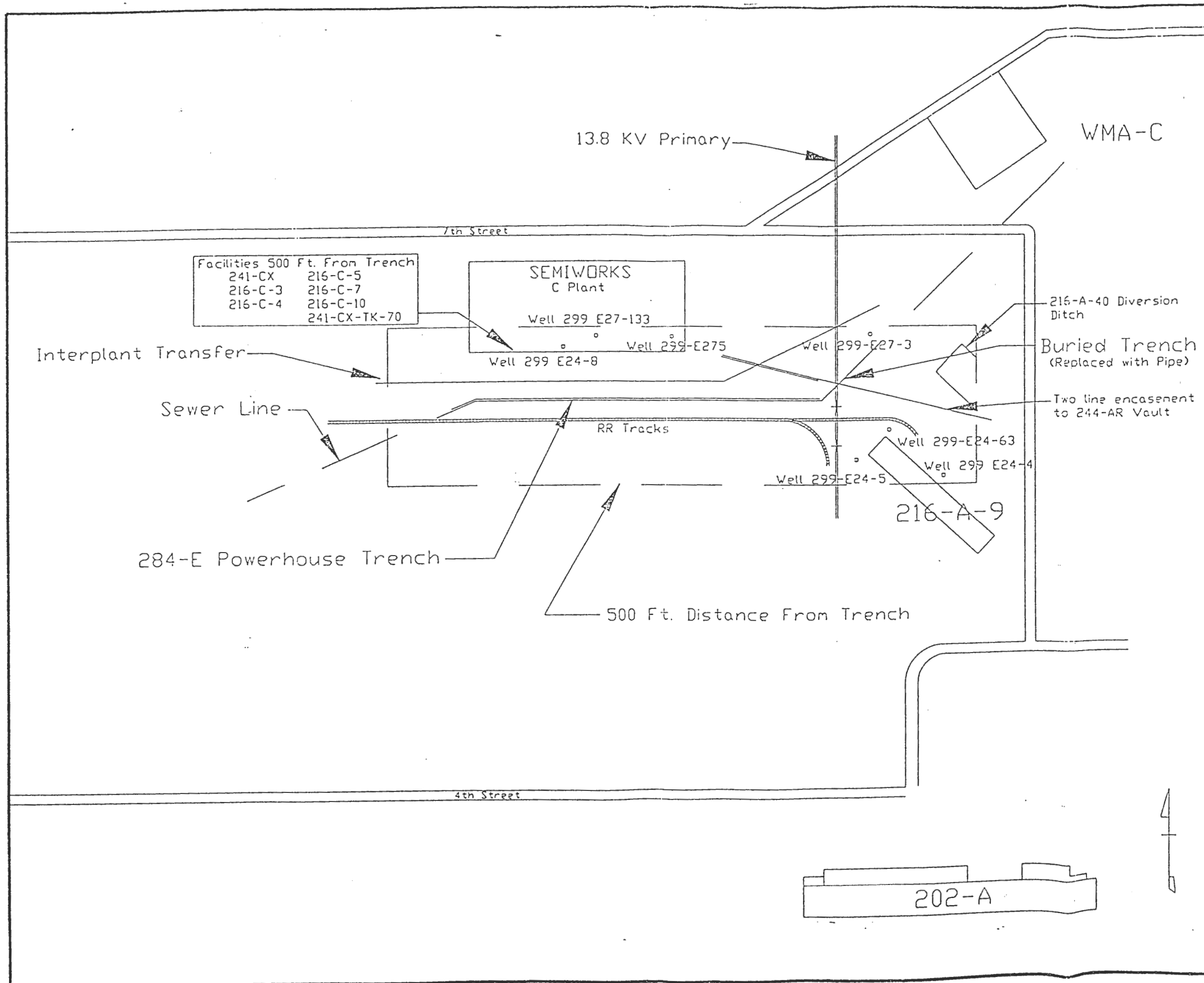
Figure 3-1 Current Trench Configuration.
