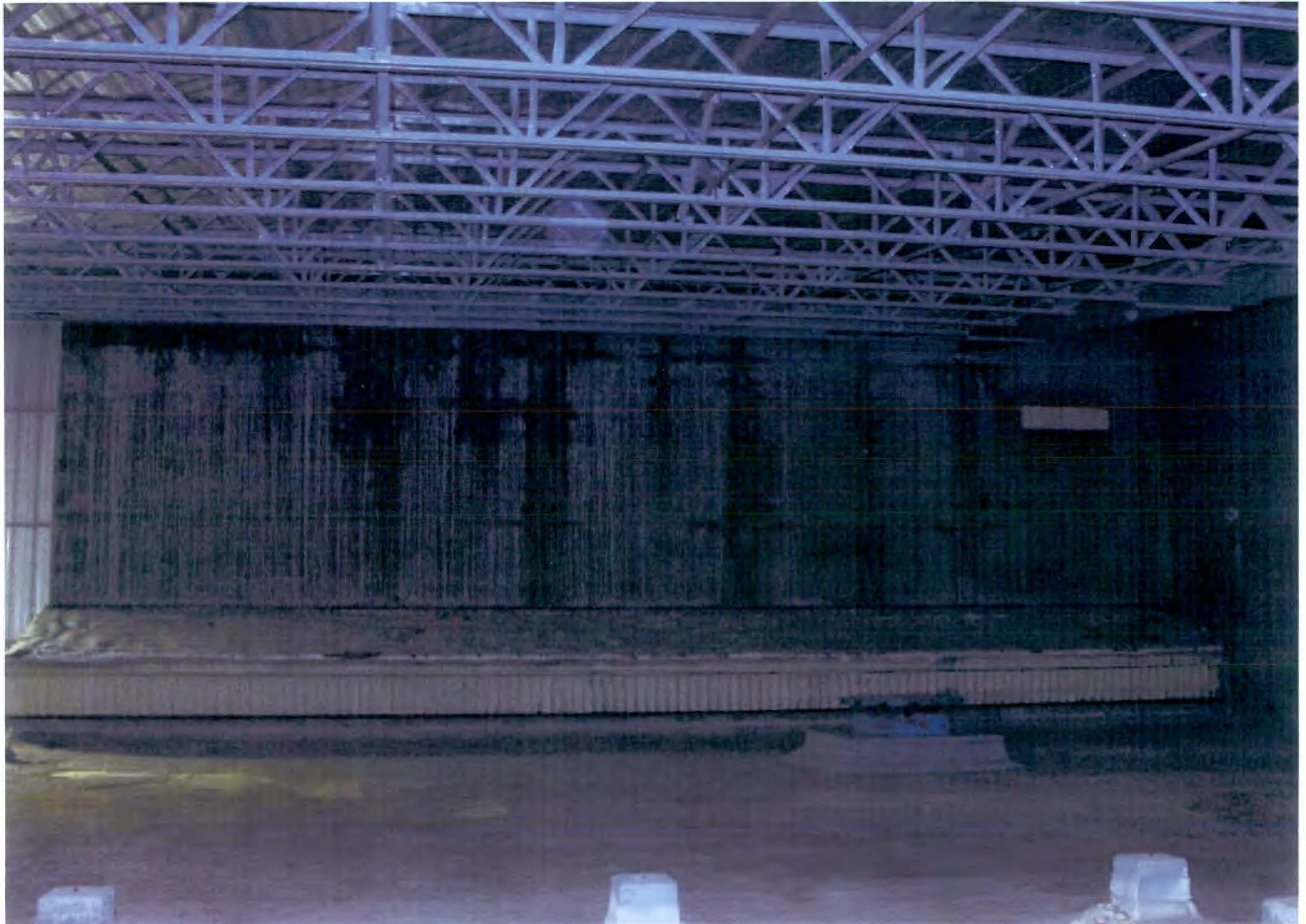
PHOTO # 112/109N/Area Under SSE Roof-N.Wall W.of Press./El.40'/02-07-2012
