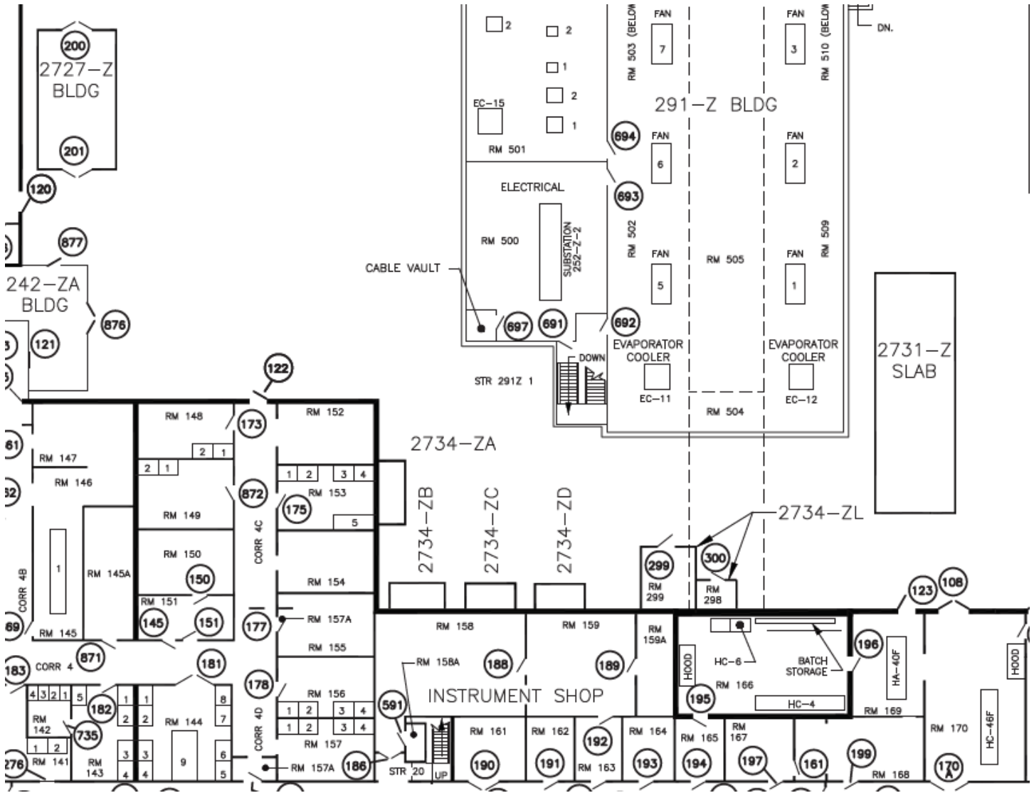
Figure 1. 2734ZD In Relation to Other Buildings
