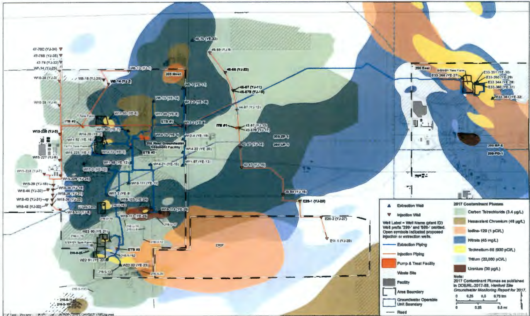
Figure B-2. 200 West P&T Well Locations and Contaminant Plumes
