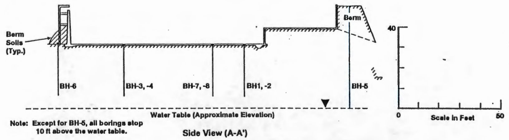
Figure 1. The 183-H Solar Evaporation Basins.
