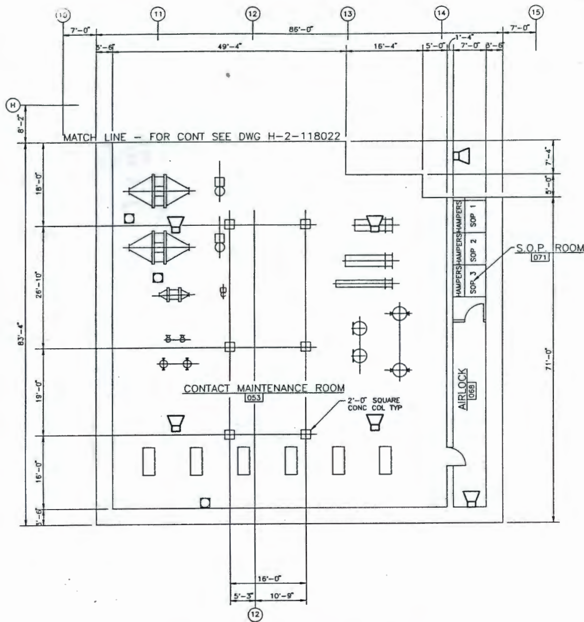
CONTACT MAINTENANCE FLOOR PLAN - EL.676'-6"
