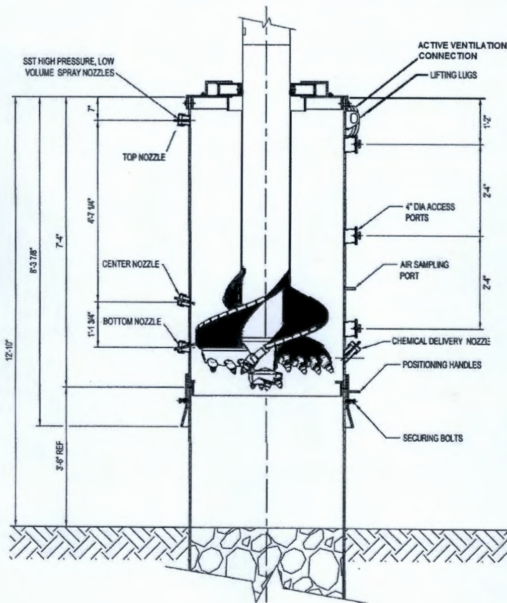
Figure 2. ATE with Auger Attached to Over-Casing.
