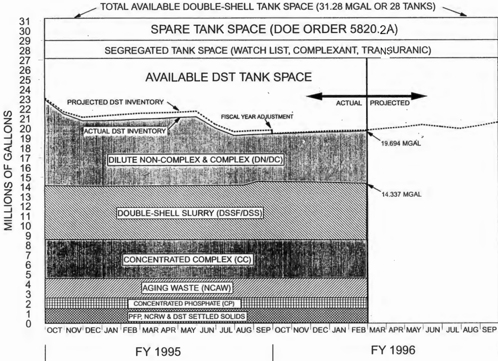
FIGURE B-1. TOTAL DOUBLE-SHELL TANK INVENTORY
