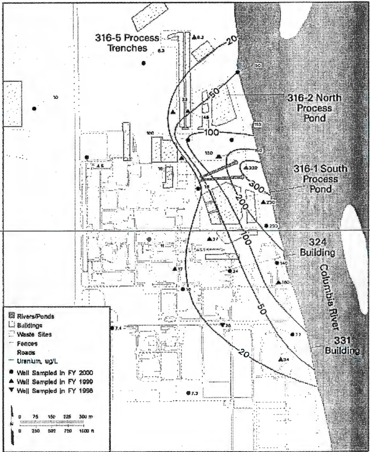
Figure 2. Average Uranium Concentration in Groundwater at 300 Area, Fiscal Year 2000.
