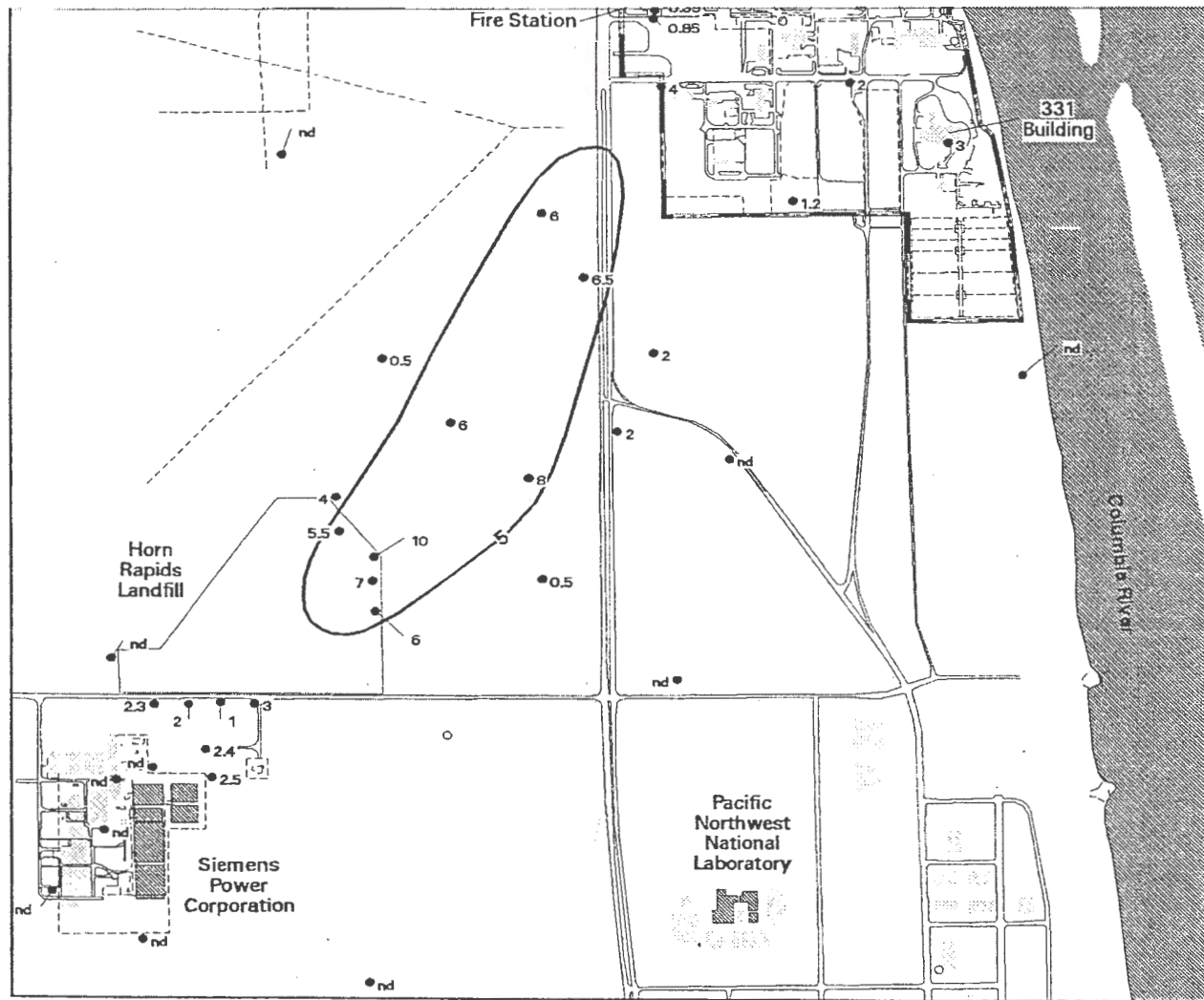
Average Trichloroethylene Concentrations for the 300 and Richland North Areas, Top of Unconfined Aquifer
